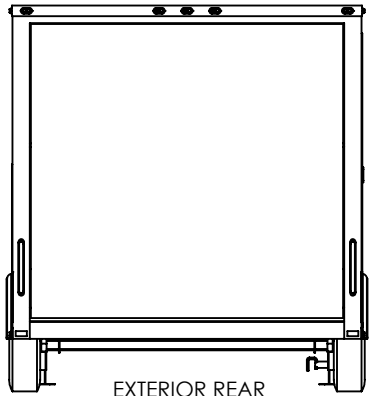
EXTERIOR REAR RAMP DOOR STANDARD SIZE 90"W x 84"H
