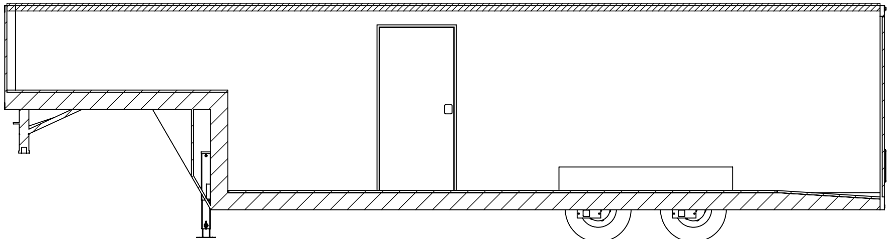
INTERIOR CURB SIDE
